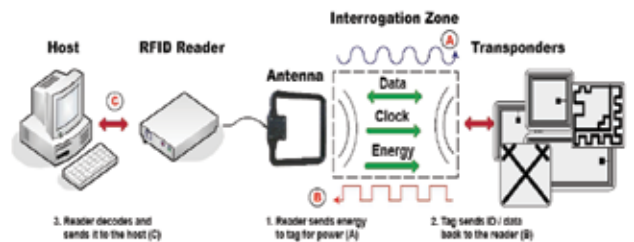
RFID design
